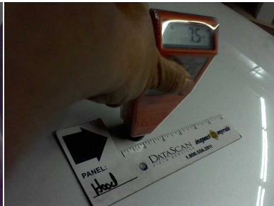
HOOD/COWL
